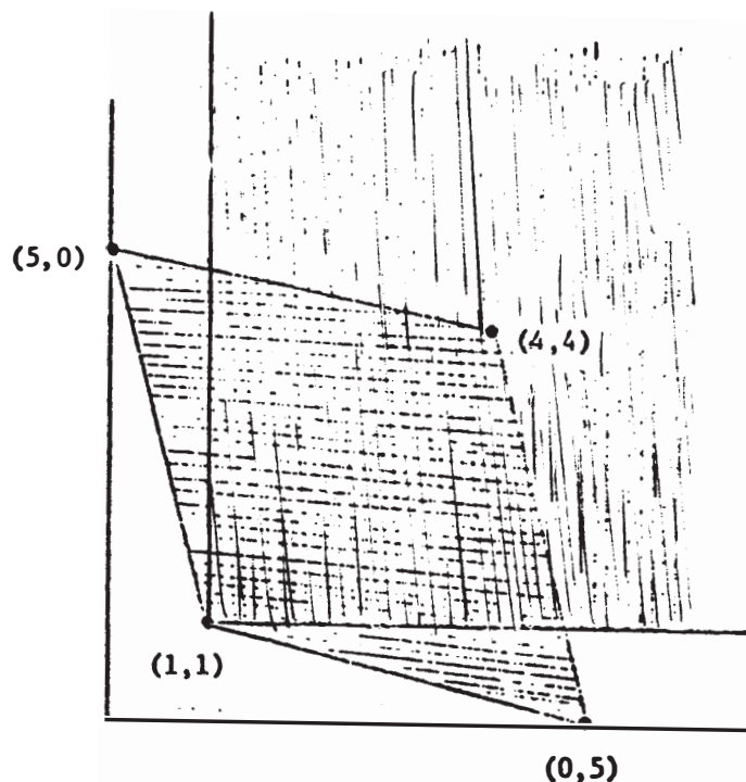
FIG. 1. Feasible and individually rational payoffs in the Prisoner's Dilemma
